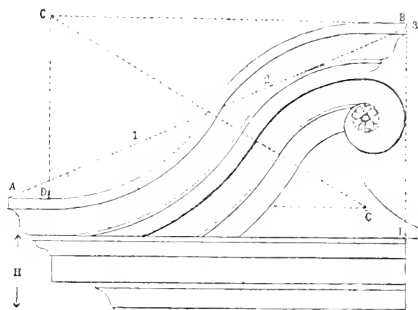
No. 52.—SETTING OUT AND FORMING COMPOUND OEGE PEDIMENT.
